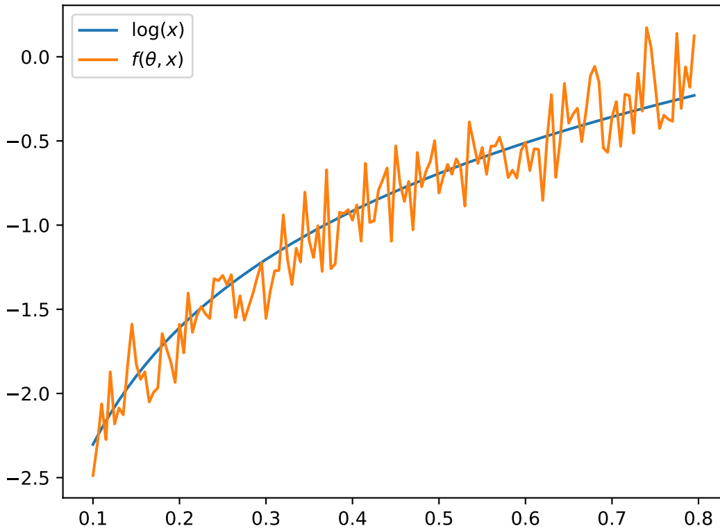
QNN inference without variance regularization
